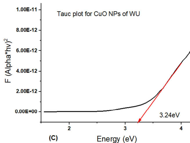
Figure 5. (a) Absorption spectrum for CuO NPs of Warburgia ugandensis (WU) at varied pH, (b) Absorption spectrum for CuO NPs of Warburgia ugandensis (WU) at varied time and (c) Tauc plot of CuO NPs.
